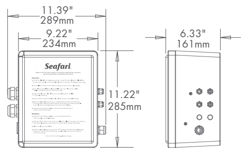
Control Box
