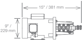
Feed Pump
