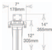
Single Post Filter
