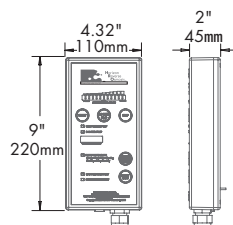
Controller Pad
